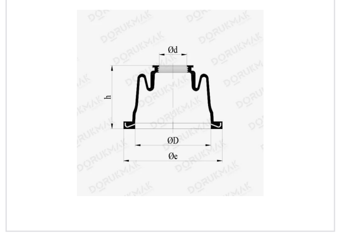
FIG. 02 Technical drawing
