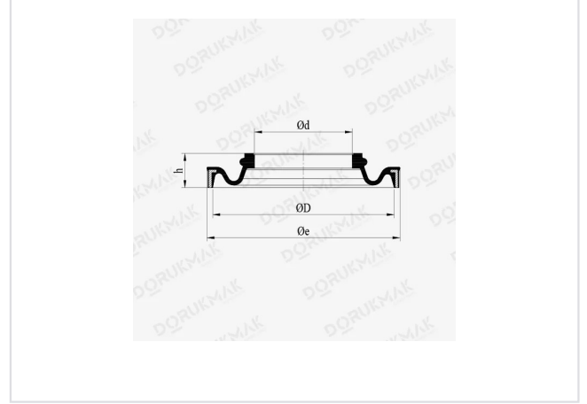
FIG. 02 Technical drawing
