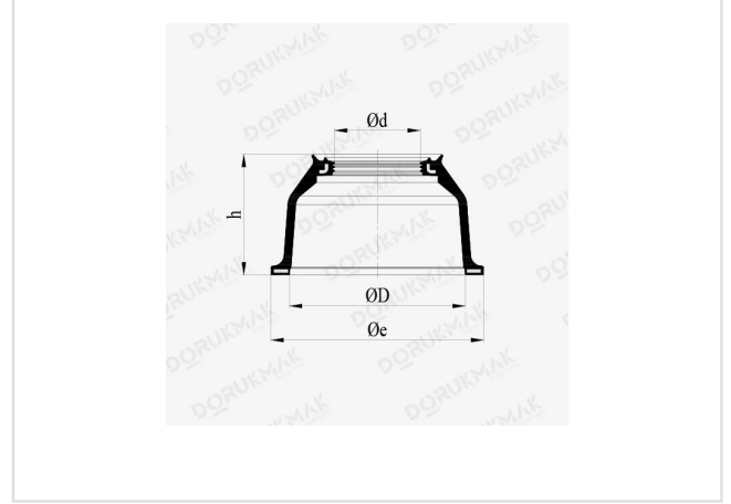
FIG. 02 Technical drawing
