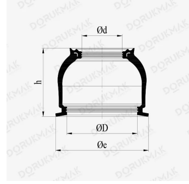
FIG. 02 Technical drawing
