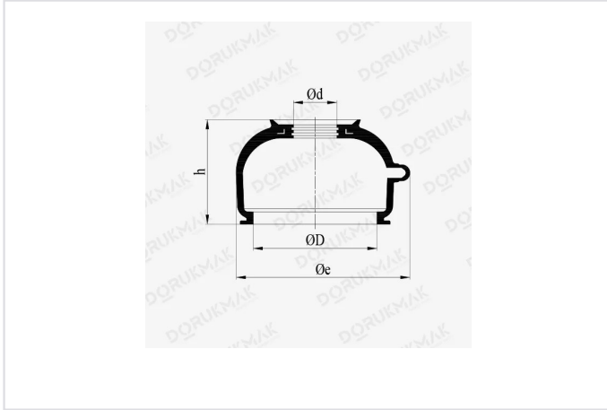
FIG. 01 Technical drawing
