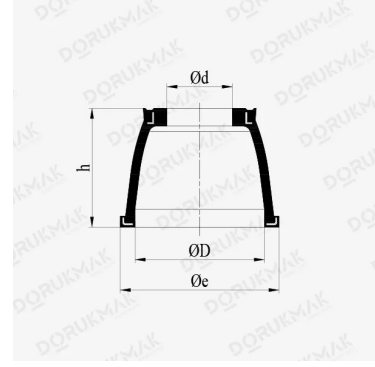
FIG. 02 Technical drawing
