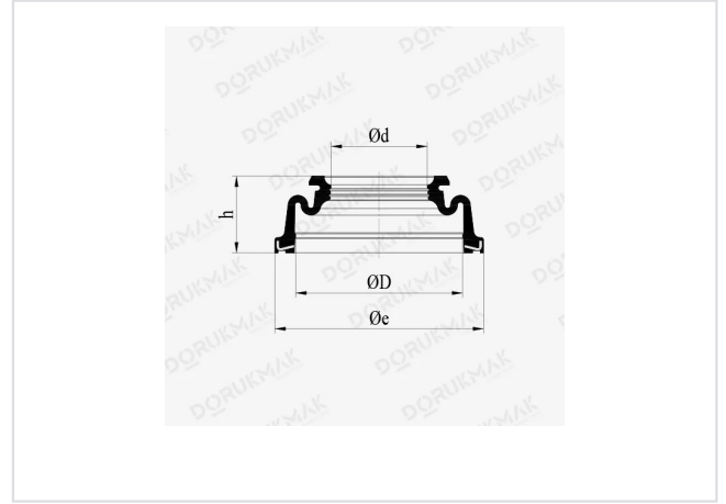
FIG. 02 Technical drawing
