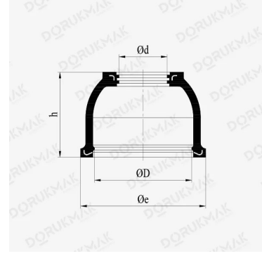
FIG. 02 Technical drawing
