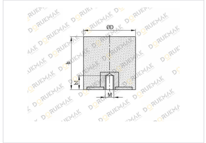
FIG. 02 Technical drawing
